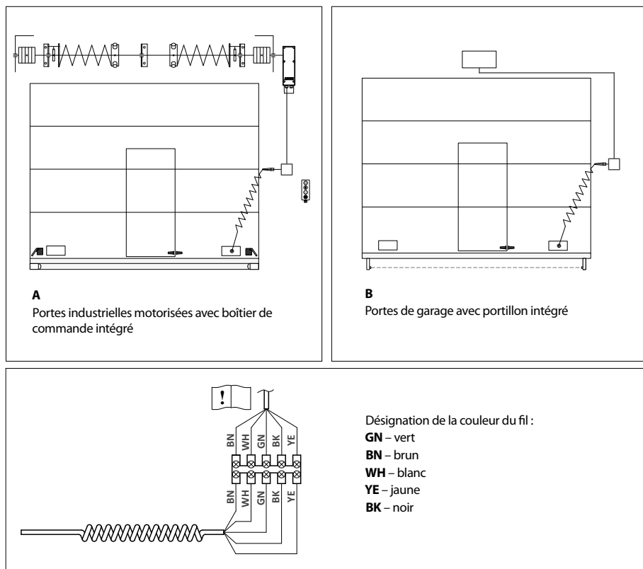
Figure 2 – Installation
