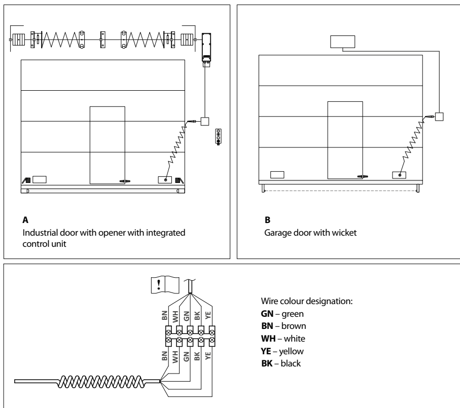
Figure 2 – Mounting
